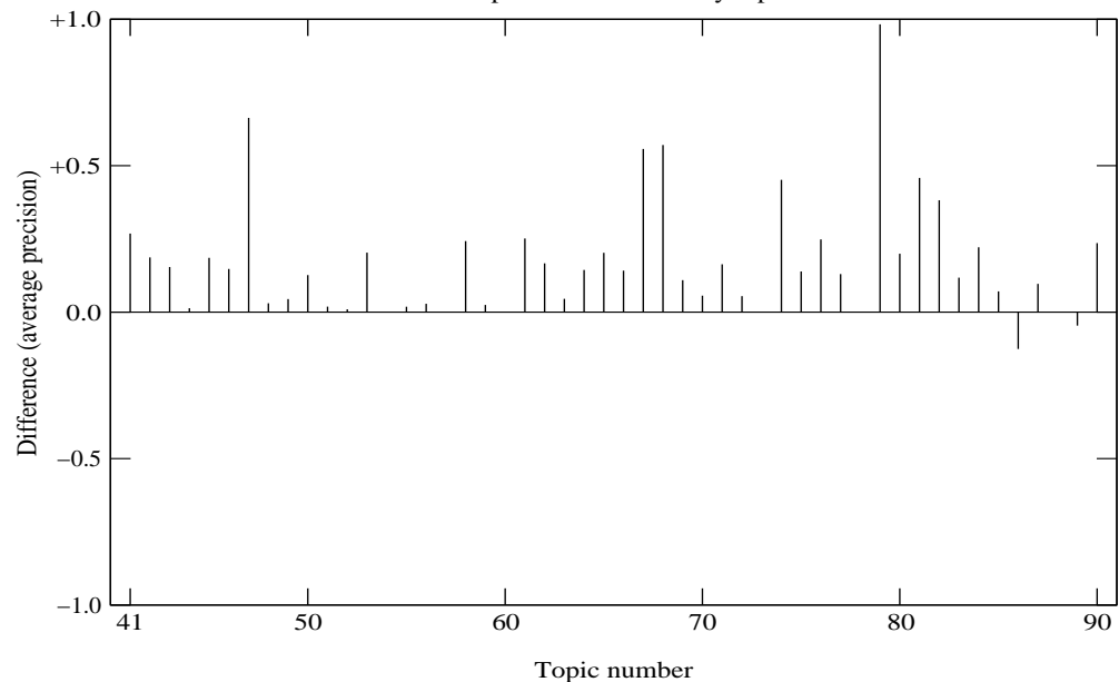
Run sinaiorg Comparison to median by topic
