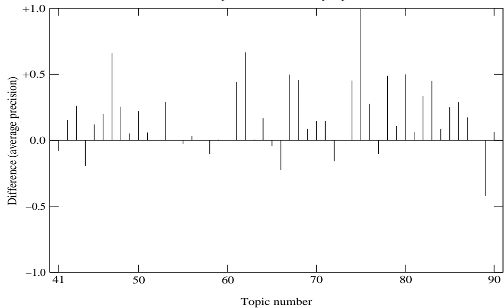
Run exeg1 Comparison to median by topic
