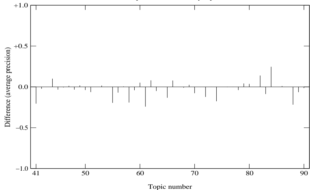
Run tlrtrtd Comparison to median by topic
