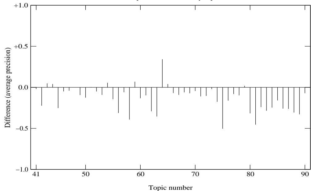
Run kcslmultitdn Comparison to median by topic
