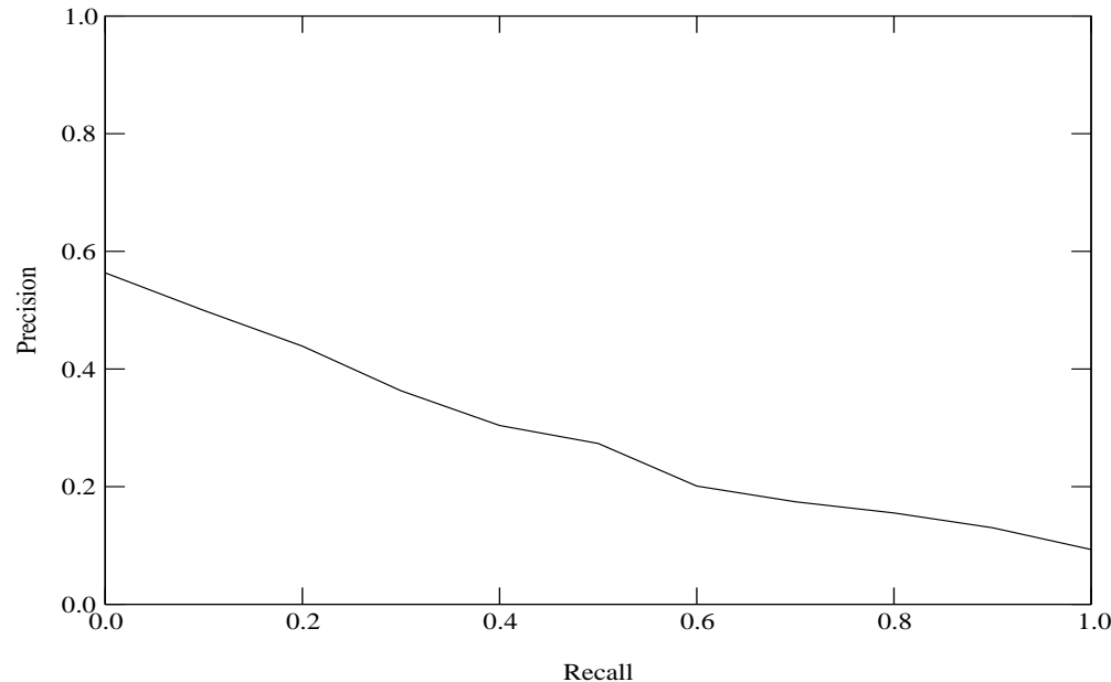
Run hkust Recall-Precision Values
